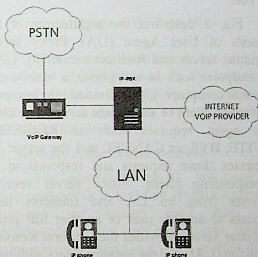
Figure 1. VOIP System
