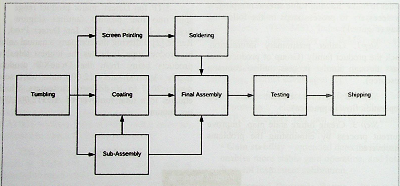
Figure 3. DyneX® Production Process Flow.
