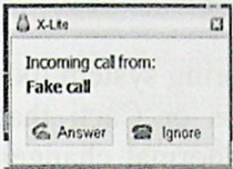
Figure 7. Invite-flood attack
