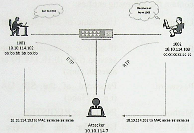
Figure 5. Eavesdropping
