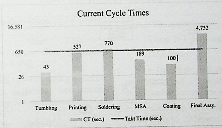
Figure 5. Current ETP production process cycle time.
