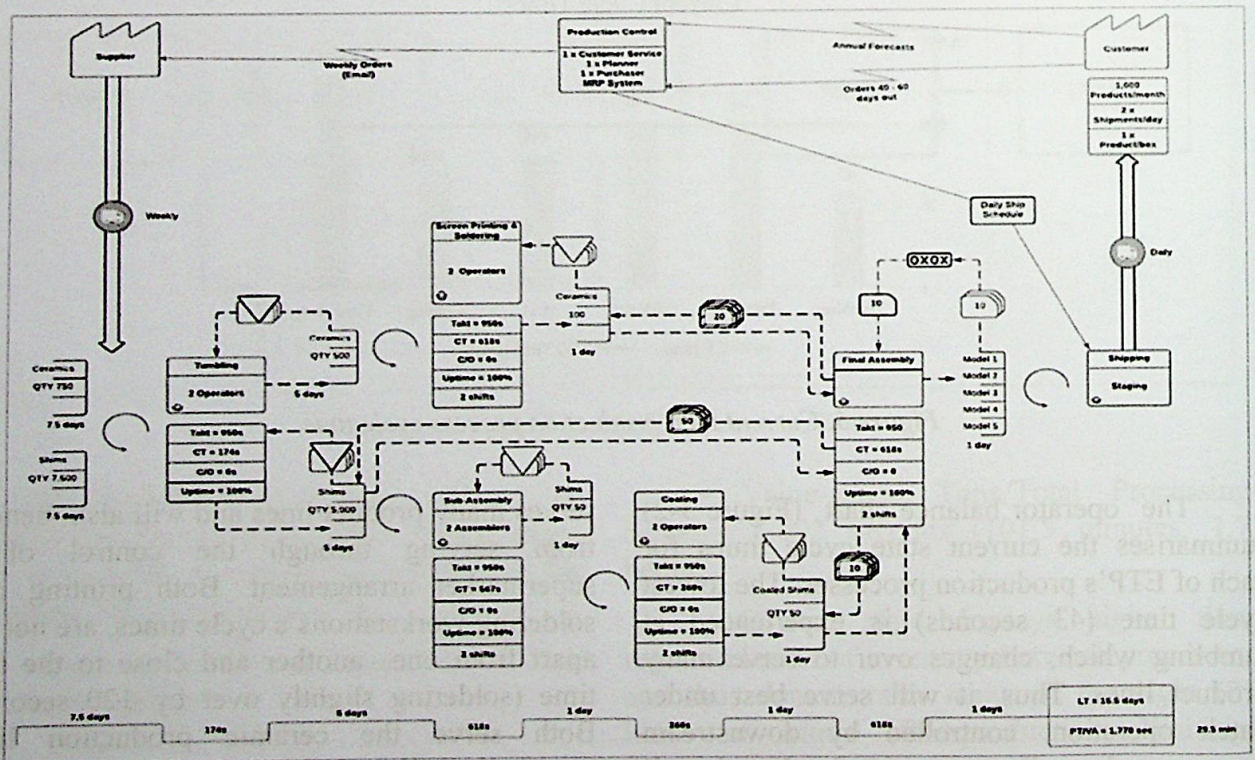
Figure 6. DyneX® Current-State Value Stream Map.
