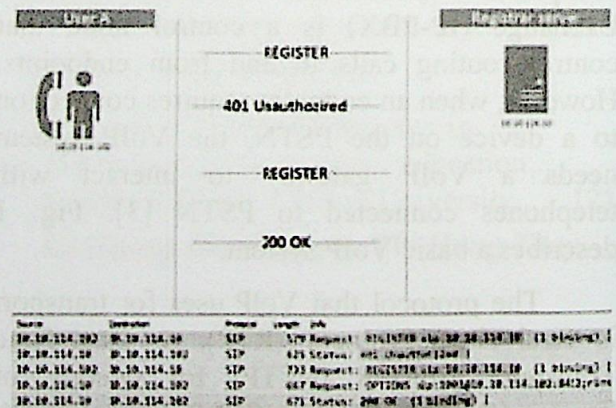
Figure 3. SIP registration process
