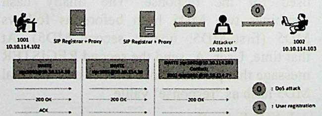
Figure 6. DoS attack
