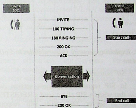
Figure 4. SIP dialog flow
